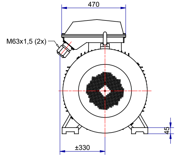
Shaft detail
