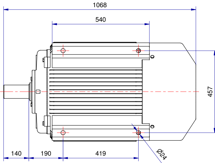
01-IP55-Cast Iron-IE4-280M B3-4_8
